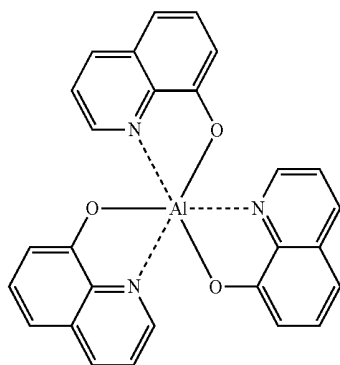
\text{Alq}_3
